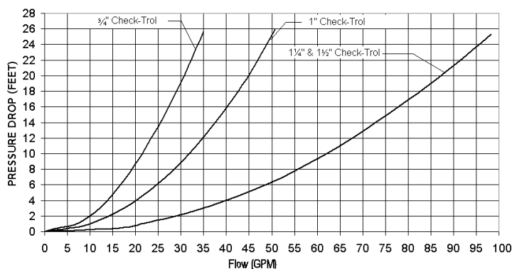
PERFORMANCE CURVE
